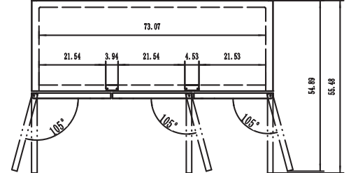
C-72RM-HC TOP VIEW
