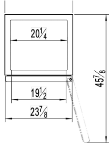
C-10RM-HC TOP VIEW
