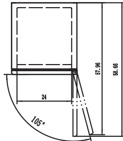
C-23RM-HC TOP VIEW
